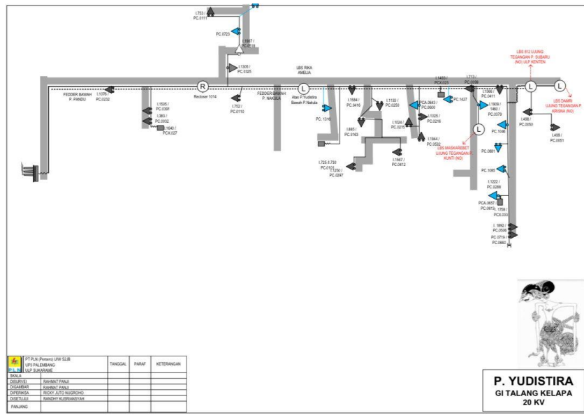
Lampiran 5 Single Line Penyalang Yudistira
