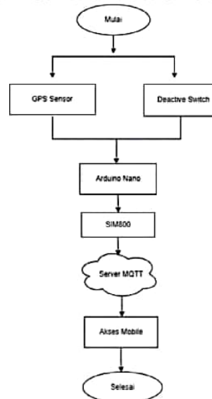
Figure 2. Hardware Design Scheme
