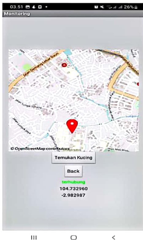
Figure 12. Monitoring Page
