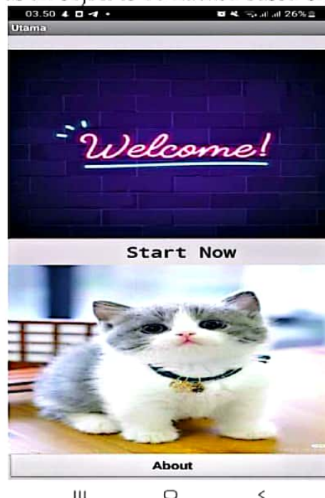
Figure 10. Home
