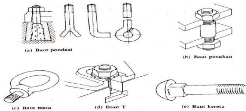
Gambar 2.13 Macam-macam baut Sumber: (13)
