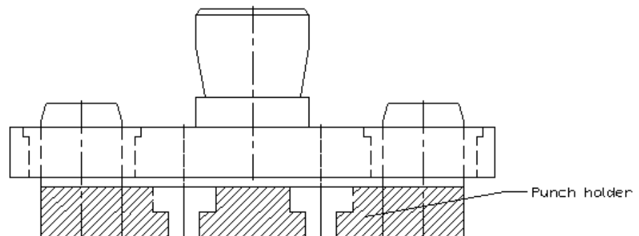
Gambar 2.19 Punch Holder
