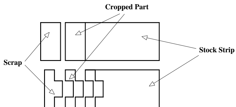
Gambar 2.10 Proses Cropping
