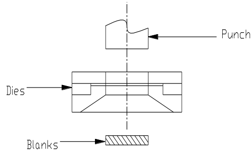
Gambar 2.5 Proses Blanking
