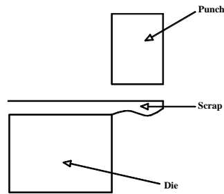
Gambar 2.8 Proses Shaving
