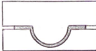
Gambar 2.16 Embossing
