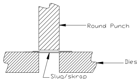
Gambar 2.4 Proses Pierching
