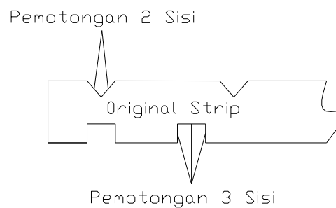
Gambar 2.6 Proses Notching
