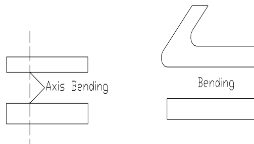
Gambar 2.12 Proses Bending
