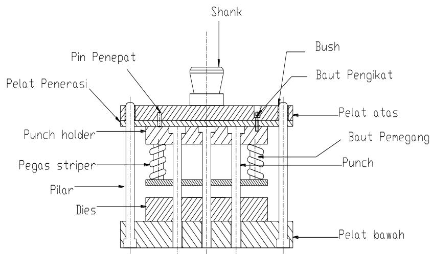
Gambar 2.3 Progressive Tool
