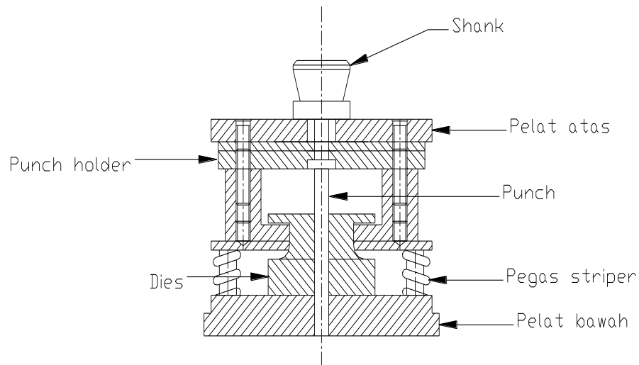
Gambar 2.2 Compound Tool
