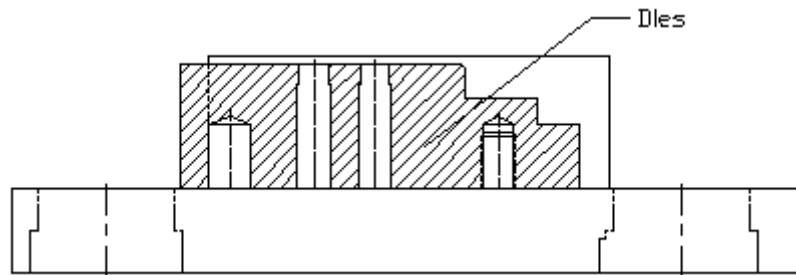
Gambar 2.21 Dies
