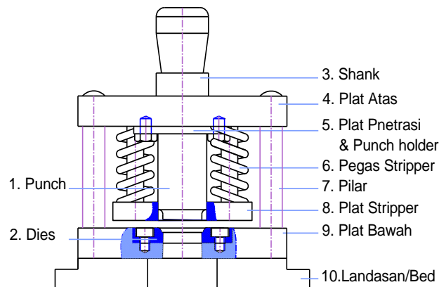
Gambar 2.1 Simple Tool
