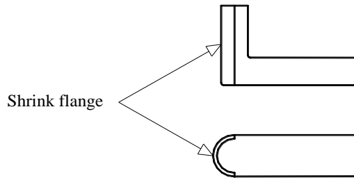
Gambar 2.13 Proses Flanging
