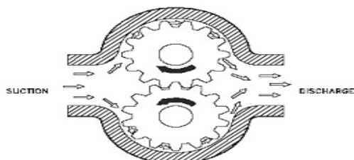
Gambar 2.2 Pompa rotary
