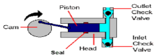
Gambar 2.1 Pompa Reciprocating
