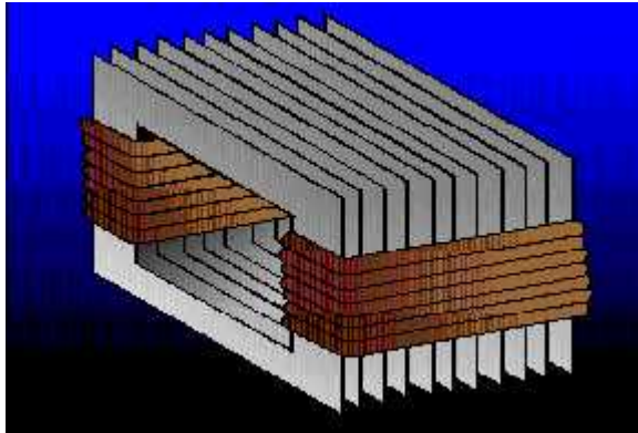
Gambar 2.9 Inti Besi Transformator
