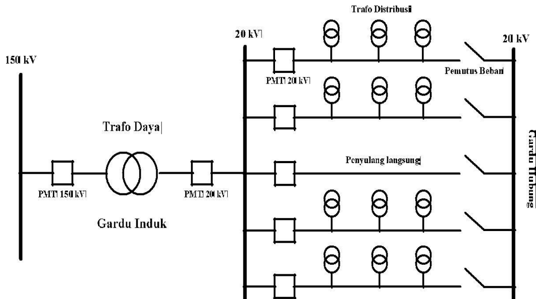
Gambar 2.5 Jaringan Distribusi Sistem Spindel
