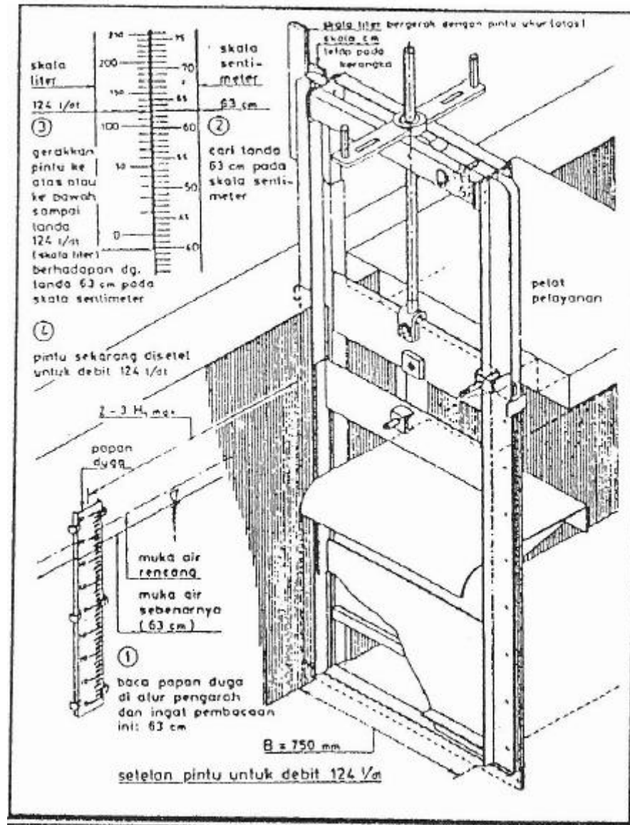
Gambar 2.3 Sketsa Isometris Alat Ukur Romiyn
