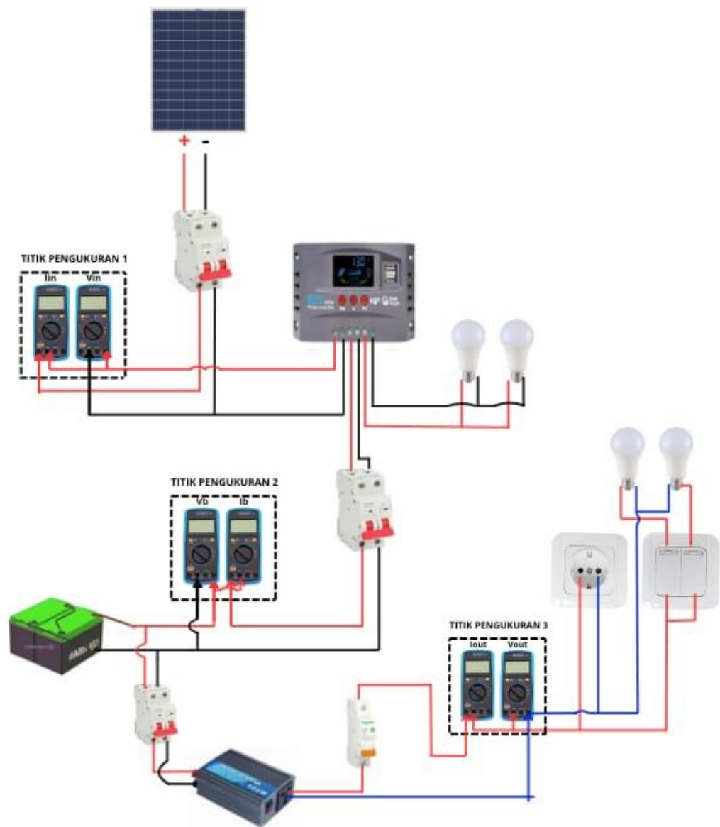
Single Line Off-Grid
