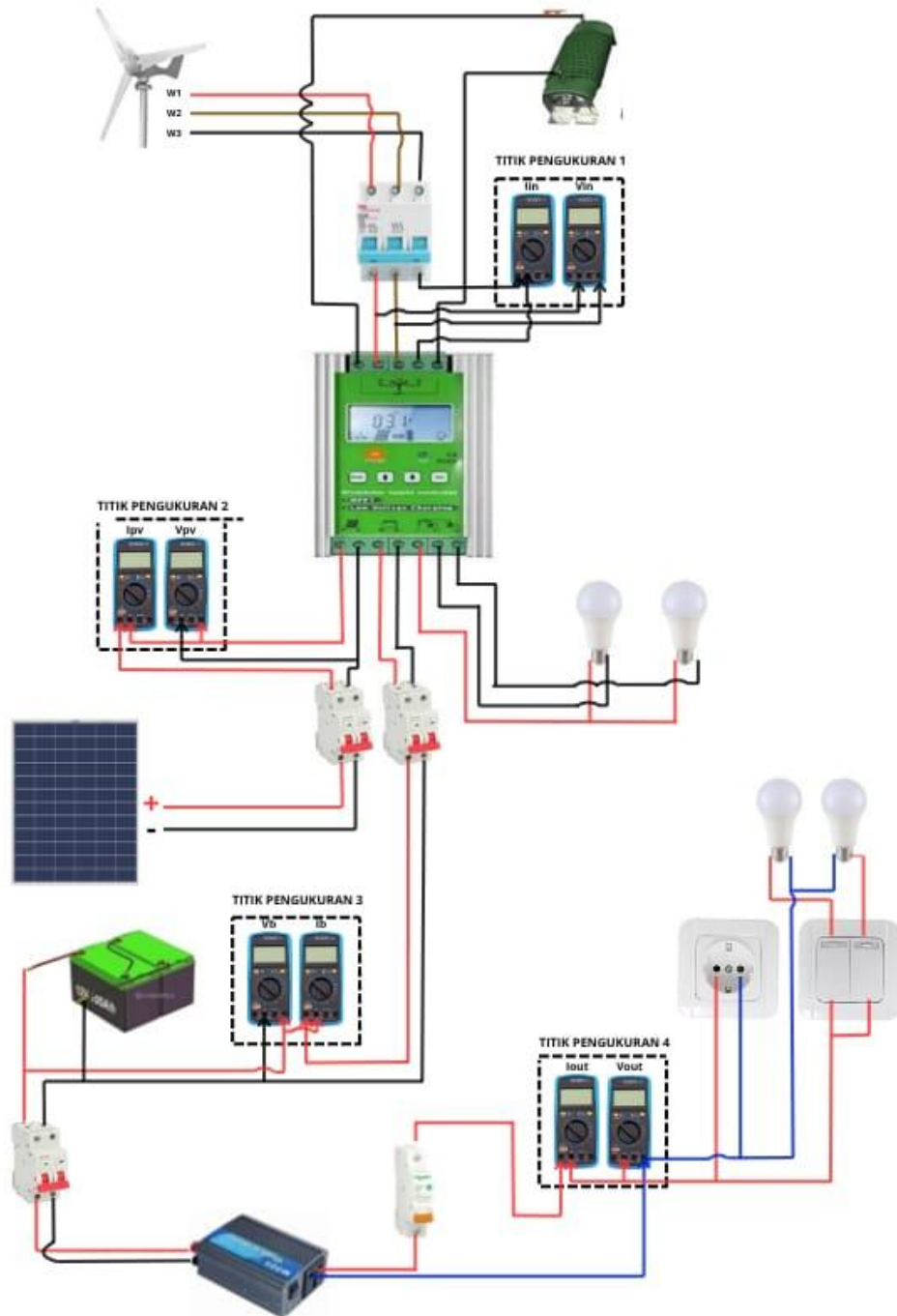
Lampiran 5 Single line Diagram
