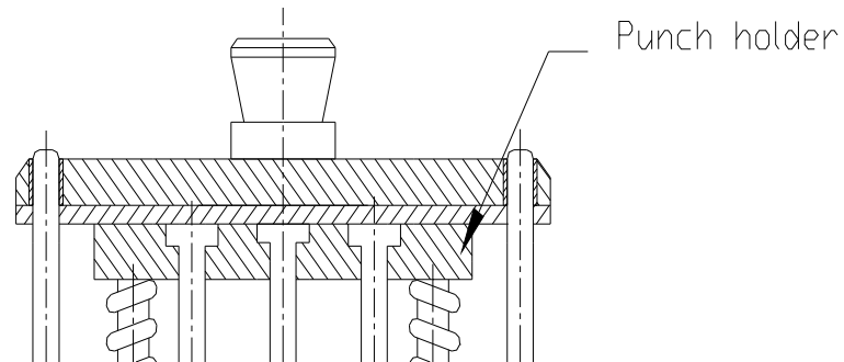
Gambar 2.9 Punch Holder
