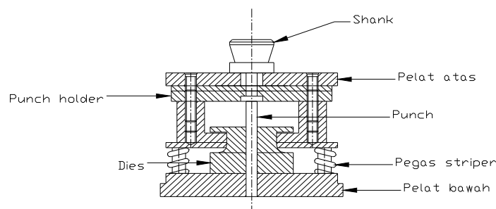
Gambar 2.4 Compound Tool
