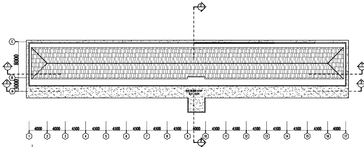
DENAH ATAP SKALA 1:250
