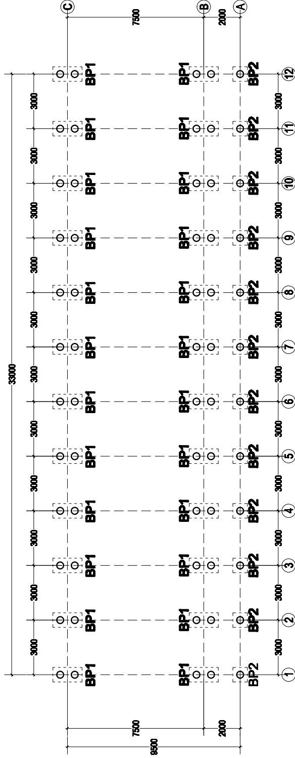
DENAH BORED PILE Scale 1:100
