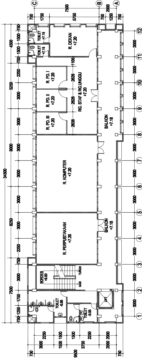
DENAH LANTAI 3 Skala 1:50
