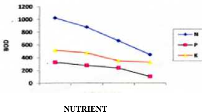
Figure 6 The relationship between the values of BOD with nutrients (NPK)
