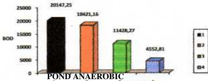
Figure 1 Relationship Between BOD value with Free anaerobic
