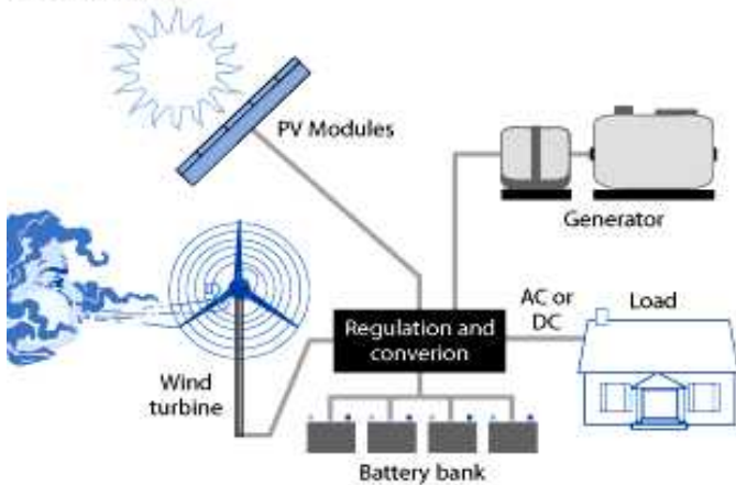
Figure 1. Hybrid system
