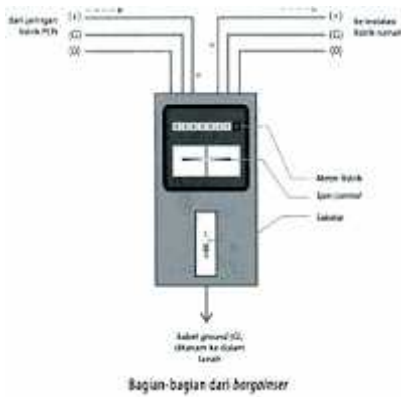
Figure 4. KWH Meter
