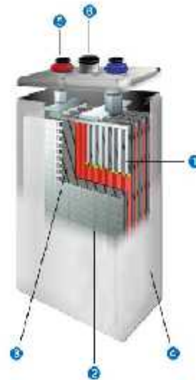
Figure 5 Battery
