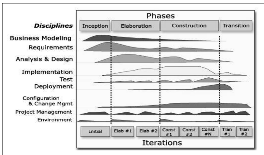
Gambar 2.2 Arsitektur Rational Unified Process
