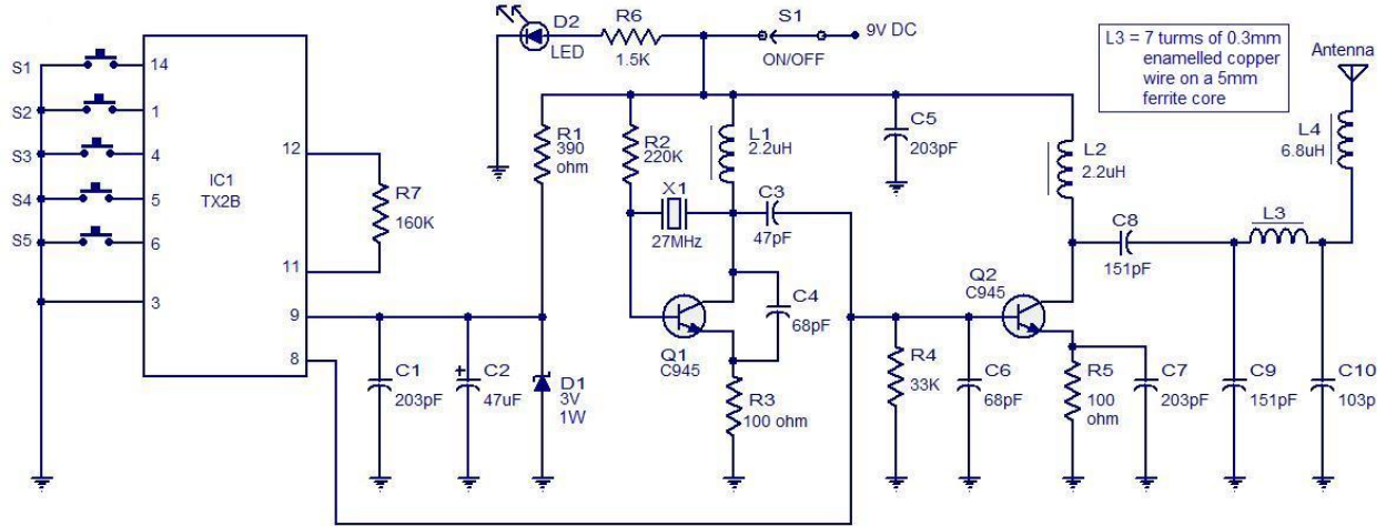
Gambar Rangkaian Transmitter Remote Control
