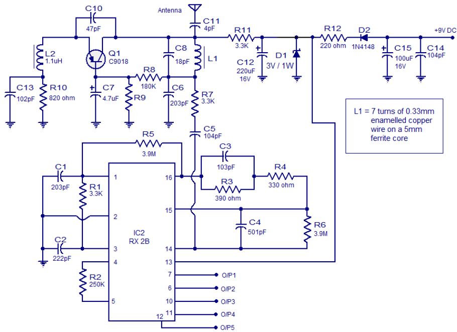
Gambar Rangkaian Receiver Remote Control
