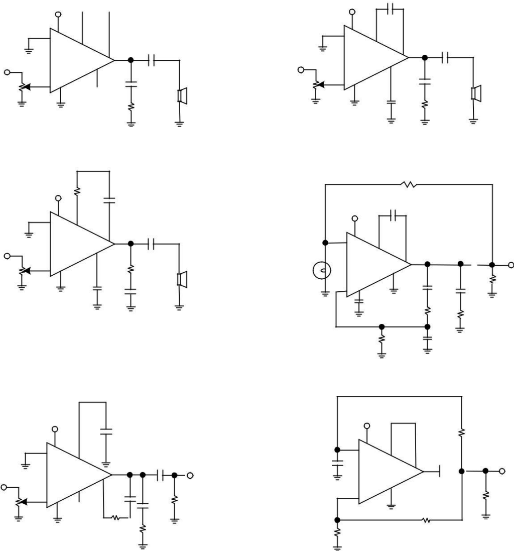
AM Radio Power Amplifier
