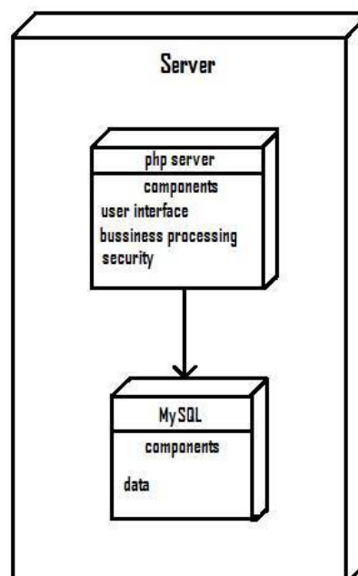
Gambar 2.4 Contoh Deployment Diagram
