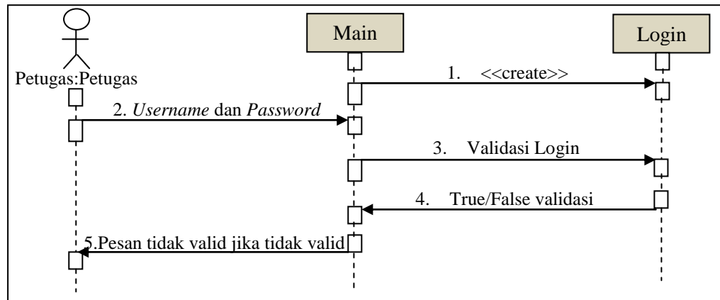
Gambar 2.3 Contoh Sequence Diagram
