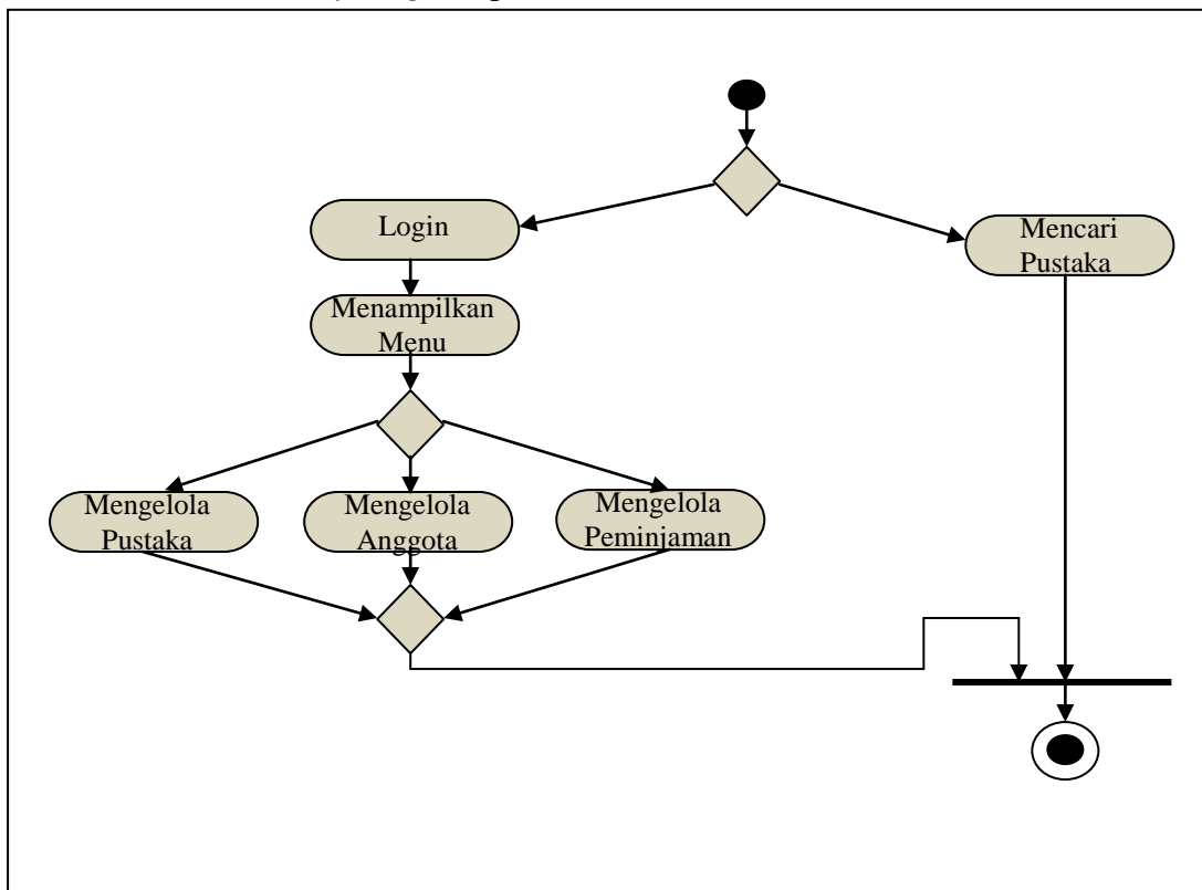
Gambar 2.2 Contoh Activity Diagram
