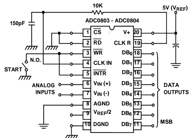
FIGURE 17. FREE-RUNNING CONNECTION
