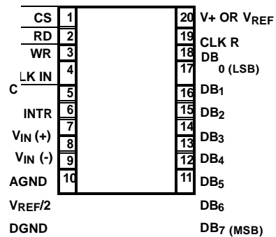
ADC0803, ADC0804 (PDIP) TOP VIEW
