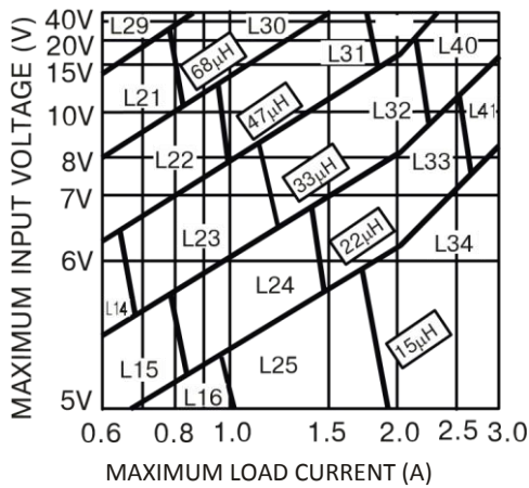
Figure 4. LM2596-3.3
