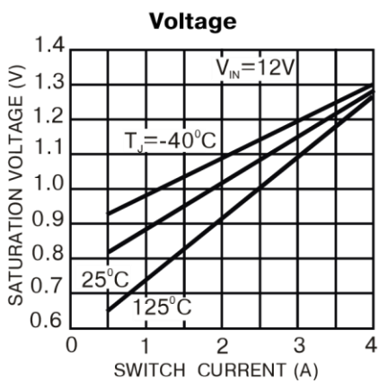
Switch Saturation
