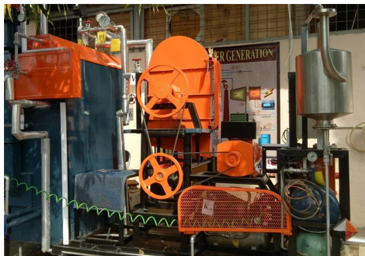
Gambar 58. Prototipe Steam Power Generator Keseluruhan
