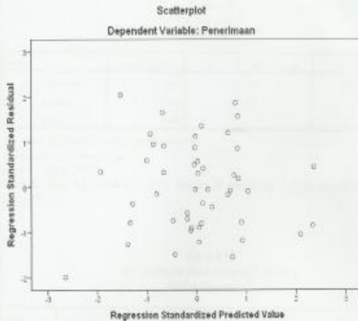
Gambar 4.3 Scatterplot
