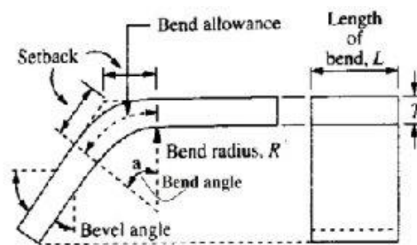
Gambar 2.1 Proses Bending (sumber: Lit. 13)
