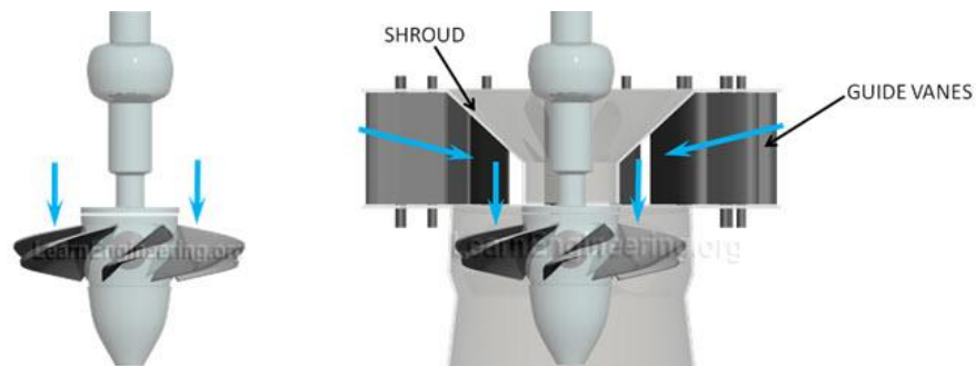
Gambar 2.6 Runner Turbin Kaplan (Sumber: Ikhsan, 2010: 17)
