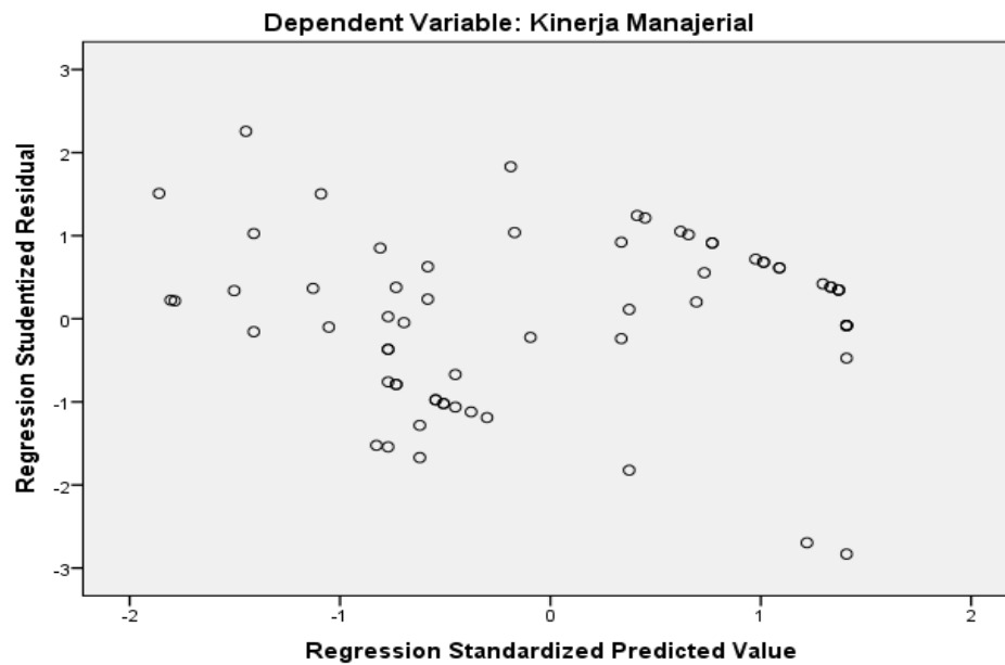
Scatterplot
