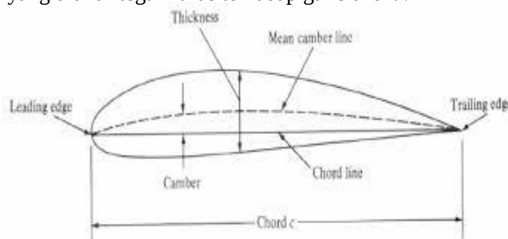
Gambar 2.12 Bagian airfoil
