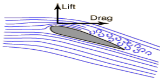
Gambar 2.10 Aliran turbulen
