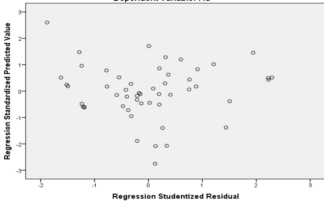
Scatterplot
