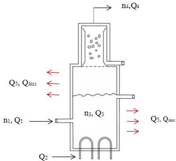
Gambar 26. Neraca Panas Water Distiller
