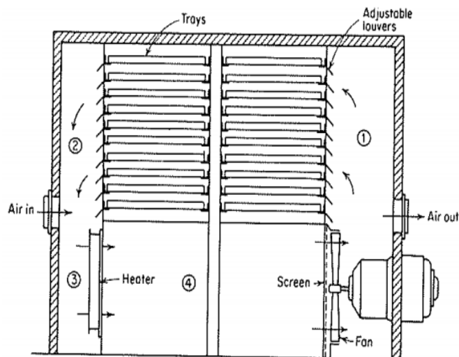
Gambar 4. Tray Dryer
