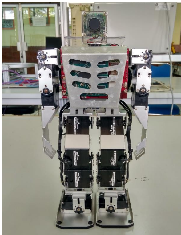
Gambar 2. 1 Robot Humanoid
