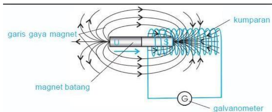
Gambar 2.5 Percobaan Faraday.
