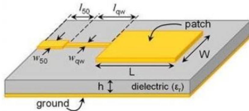
Gambar 2.6 Dasar Antena Mikrostrip (PCB double layer) [3].
