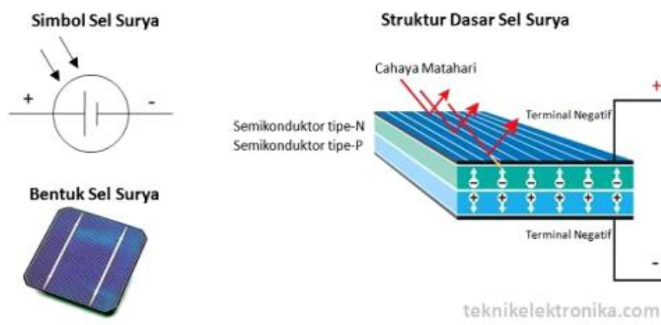
Gambar 2.4. Solar Cell [8]
