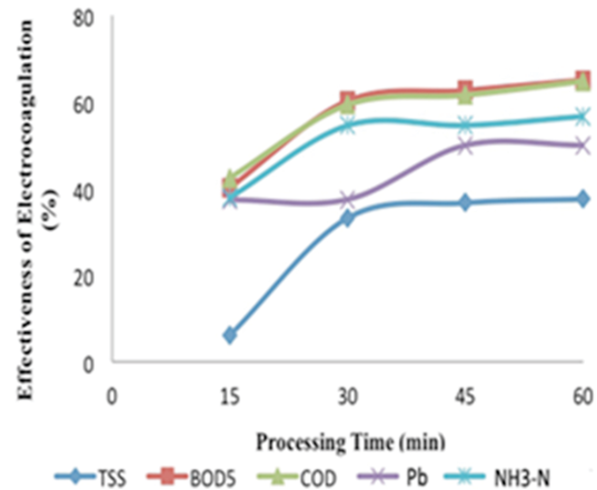
Fig. 10. Effectiveness of electrocoagulation to processing time on current density 70 A/m^2
