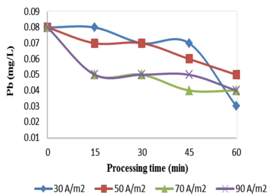
Fig. 6. The effect of current density to processing time for Pb metal
