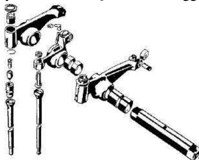
Gambar 2.14 Rocker Arm
