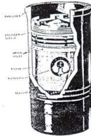
Gambar 2.29 Dinding Silinder
