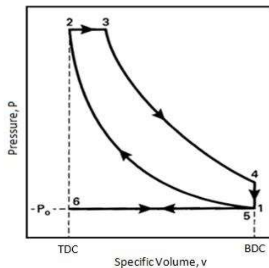
Gambar 2.1 Siklus Diesel Diagram P-V (Samlawi 2015)
