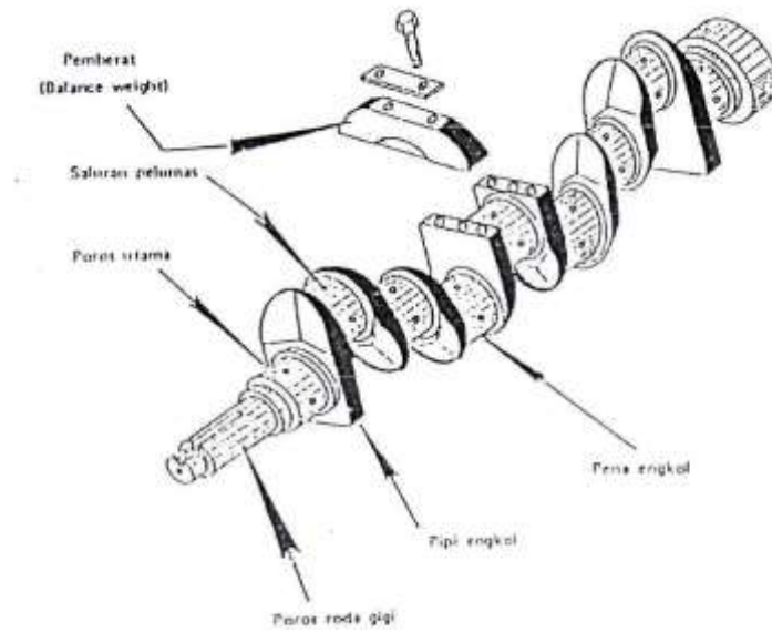
Gambar 2.20 Poros Engkol
