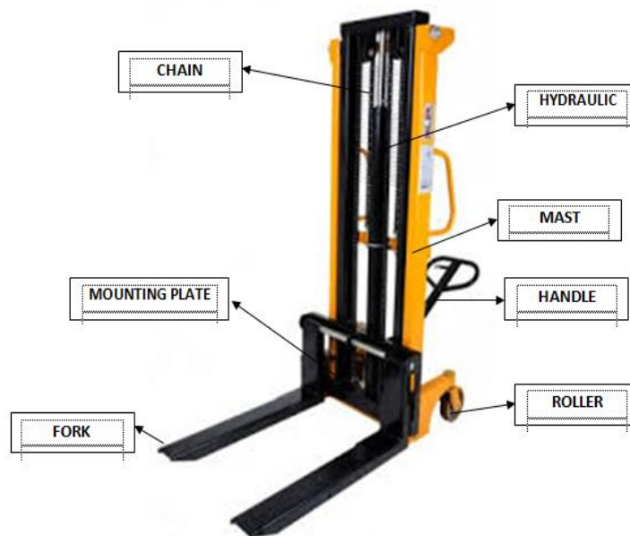
Gambar 2.1 Bagian-Bagian Portable Forklift
