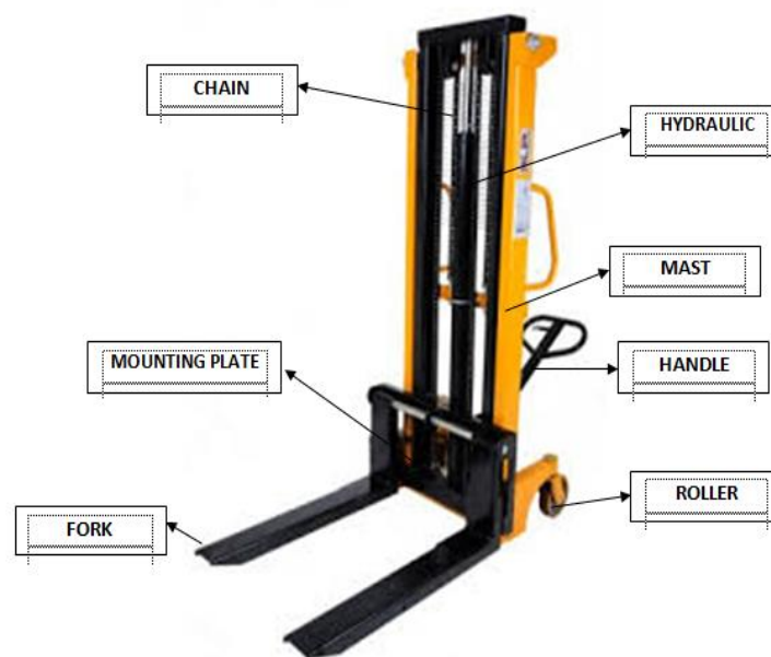
Gambar 2.1 Bagian-Bagian Portable Forklift (Sumber: Google)
