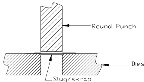
Gambar 2.4 Proses Pierching
