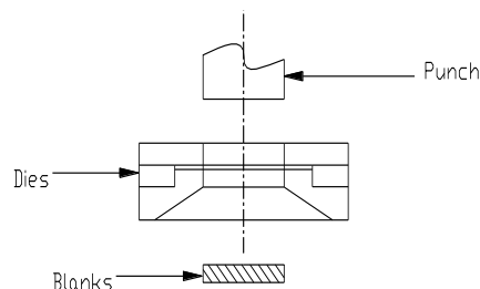
Gambar 2.5 Proses Blanking
