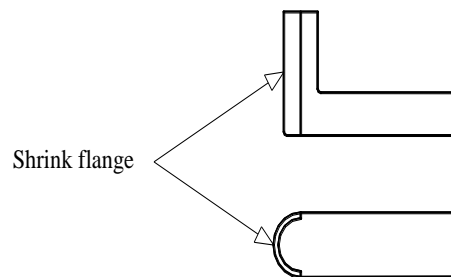
Gambar 2.13 Proses Flanging
