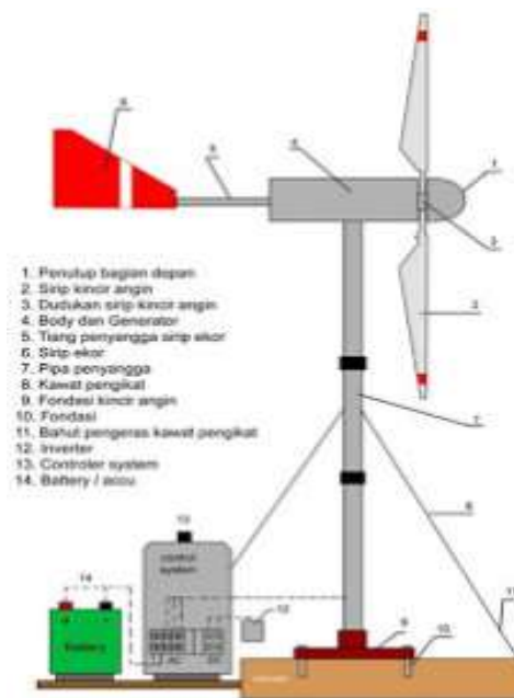
Gambar 2.3 Turbin Angin 1
