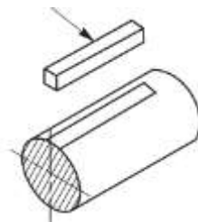
Gambar 2.8 pasak poros 3
