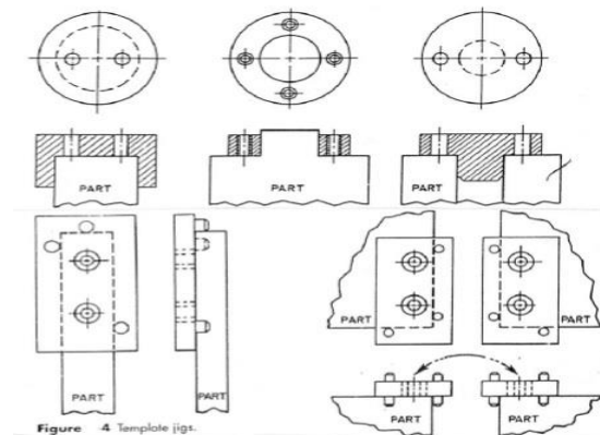
Gambar 2.1 Jig Template
