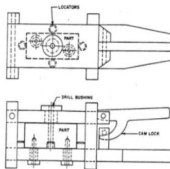
Gambar 2.6 Rotary Jig
