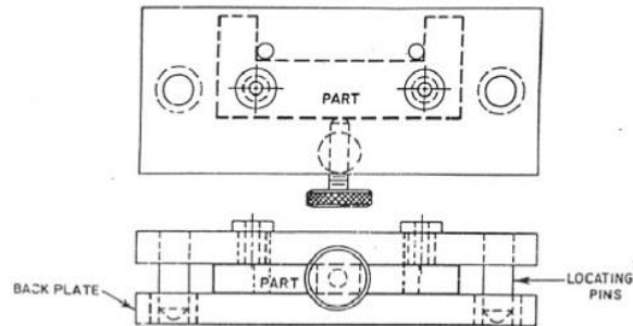
Gambar 2.3 Sandwich Jig
