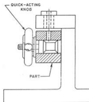
Gambar 2.4 Angle Plate Jig
