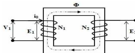
Gambar 2.1 Diagram dasar transformator
