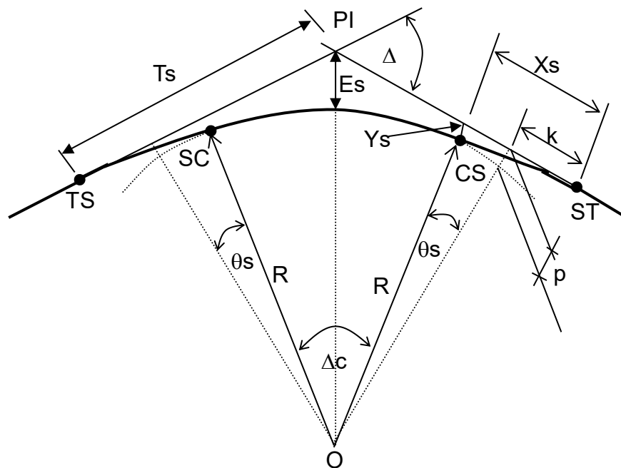
Gambar 2.5 Tikungan Spiral Circle Spiral
