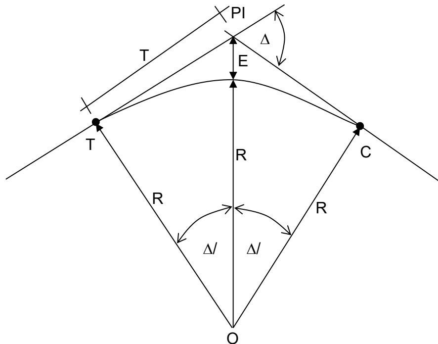
Gambar 2.4 Tikungan Full Circle
