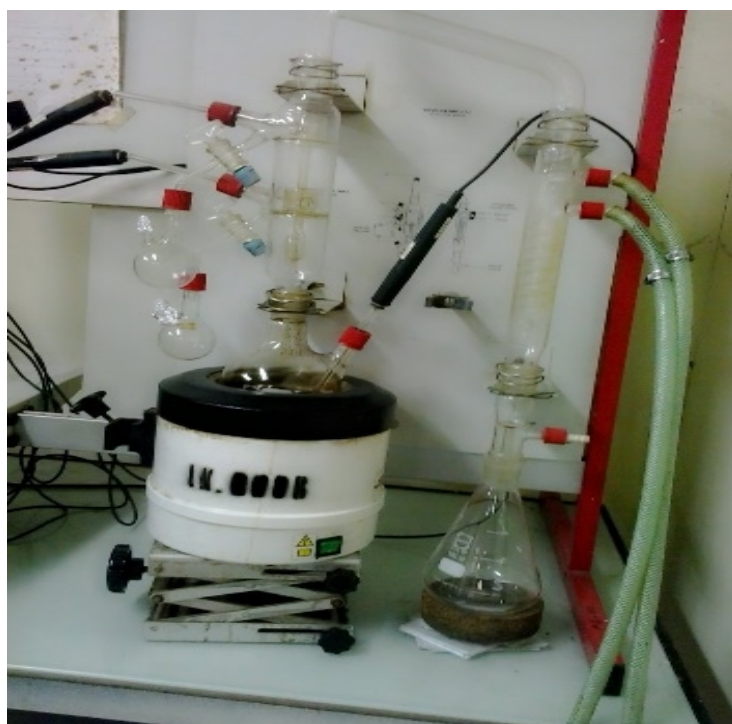
Alat Distilasi Crude Oil
