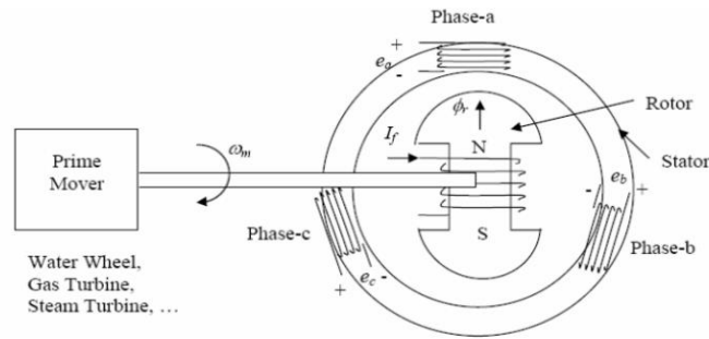
Gambar 2.2 Prinsip Kerja Generator Sinkron 5
