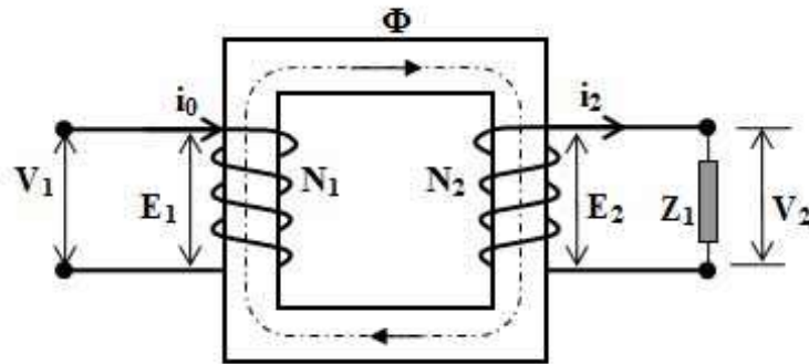
Gambar 2.5 Transformator Berbeban
