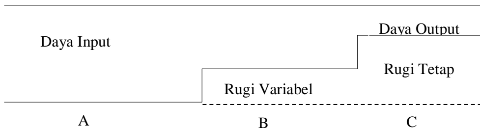
Gambar 2.20 Rugi-rugi Transformator
